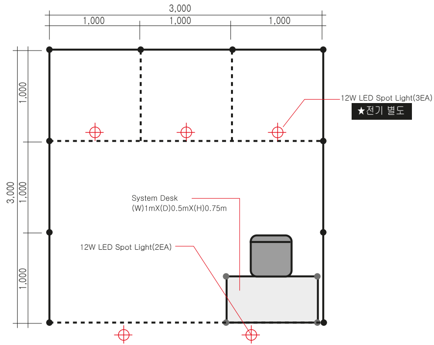
▲ Top View
